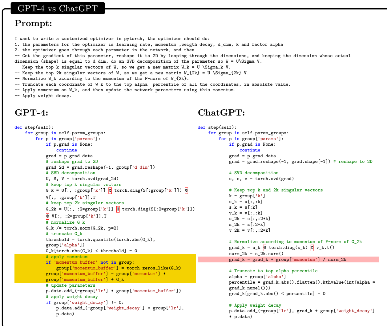
Figure 3.4: GPT-4 vs ChatGPT at implementing a customized Pytorch optimizer module. We highlight the astuteness of GPT-4 vs the mistake by ChatGPT at ‘applying momentum’.
