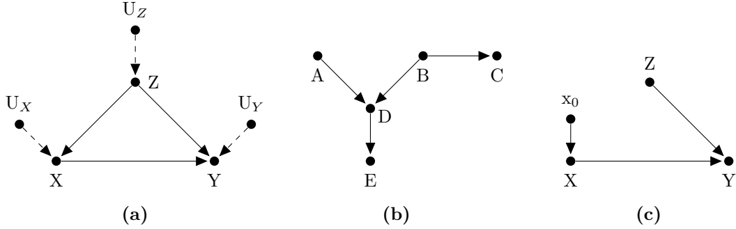
Figure 2.: (a) Directed acyclic graph corresponding to the SCM in equation (2.1) with background variables U_i explicitly depicted. (b) Graphical illustration of d -separation. D acts as a collider that opens up the path between A and C , whereas B blocks it. (c) Post-intervention graph of (a) for do(X = x_0) .
