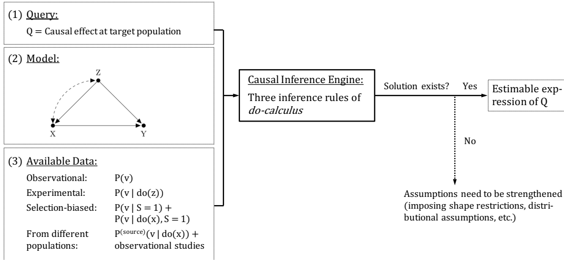
Figure 1.: Schematic illustration of the data fusion process. The causal inference engine provided by do-calculus takes three inputs: (1) a causal effect query Q , (2) a model G , and (3) the type of data, P(v|\cdot) , that is available. It is guaranteed to return a transformation of Q , based on G , that is estimable with the available data, whenever such a solution exists.
