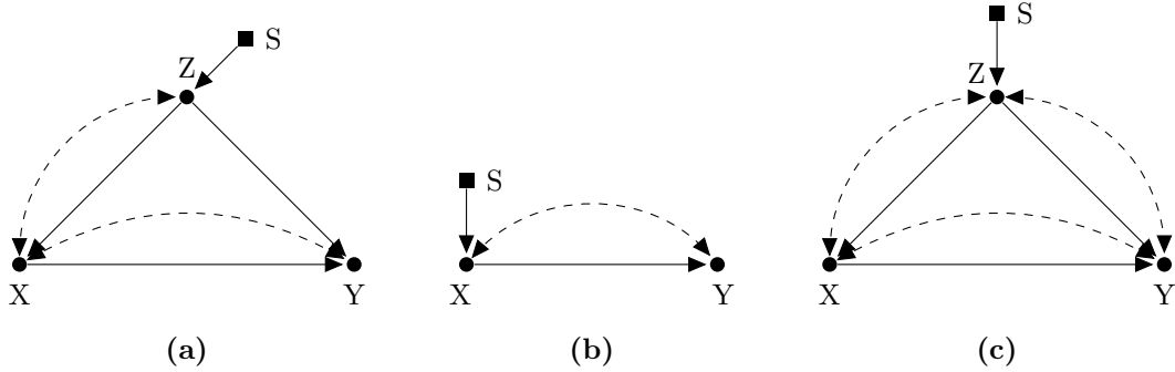
Figure 8.: (a) Z d -separates S and Y in D_{\bar{X}} . The causal effect of X on Y is thus transportable. (b) If S -nodes are only pointing into X , the causal effect P^*(y|do(x)) is directly transportable. (c) Compared to (a), a single additional unobserved confounder between Z and Y prevents transportability.
