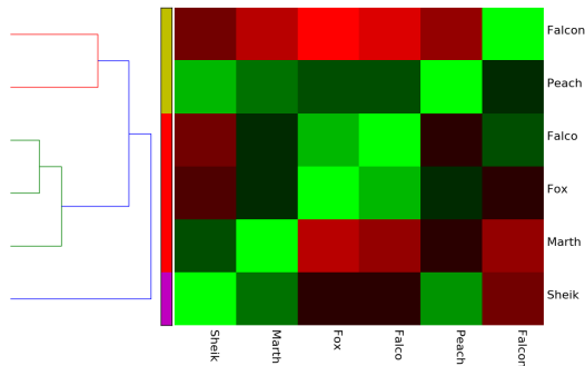
Figure 3: Hierarchical clustering of the characters by transfer time. Fox and Falco, considered to be “clone” characters, cluster tightly together.
