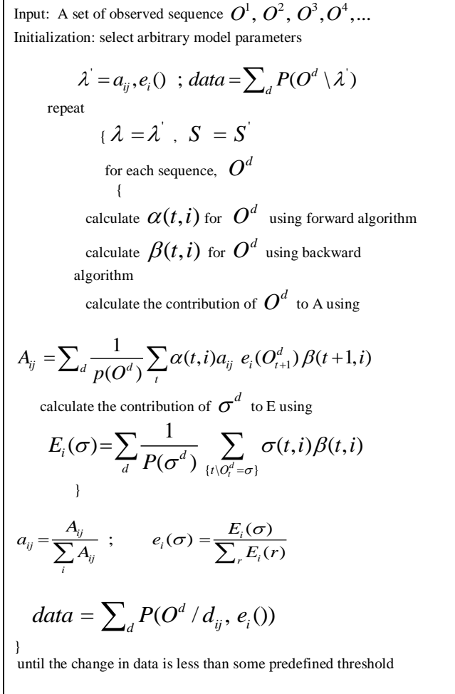
Figure 1: Baum-Welch Algorithm
